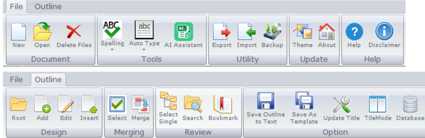
Ribbon menu
